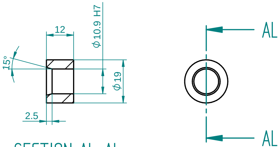
SECTION AL-AL
