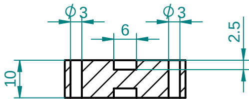
SECTION AH-AH
