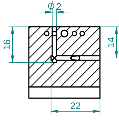
SECTION W-W
