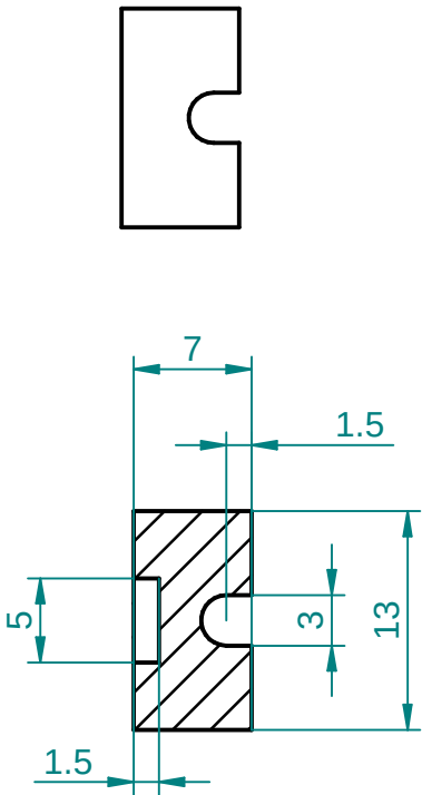
SECTION O-O
