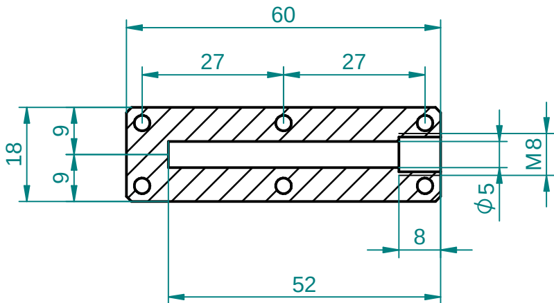
SECTION AD-AD
