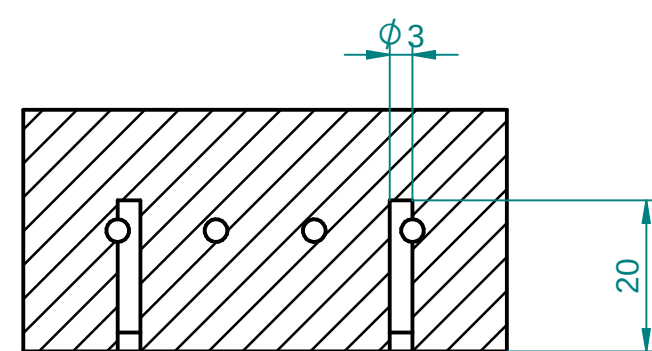
SECTION Q-Q
