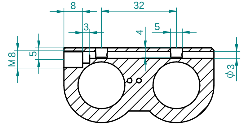
SECTION Y-Y
