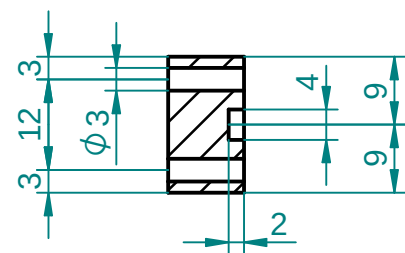
SECTION AE-AE
