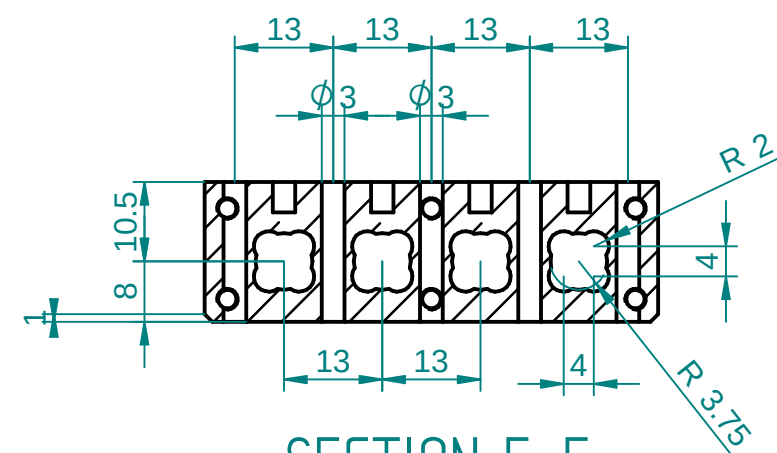
SECTION F-F
