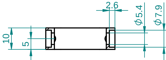
SECTION AI-AI
