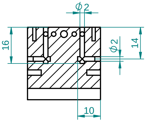
SECTION X-X
