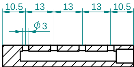
SECTION K-K
