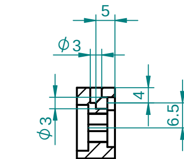
SECTION M-M
