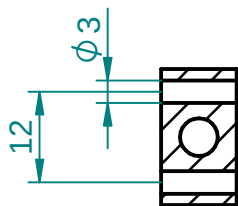
SECTION AF-AF
