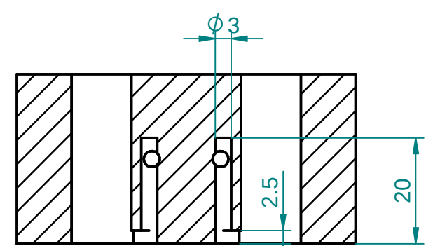
SECTION P-P
