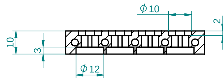
SECTION I-I
