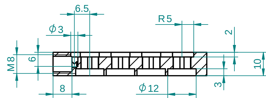
SECTION J-J
