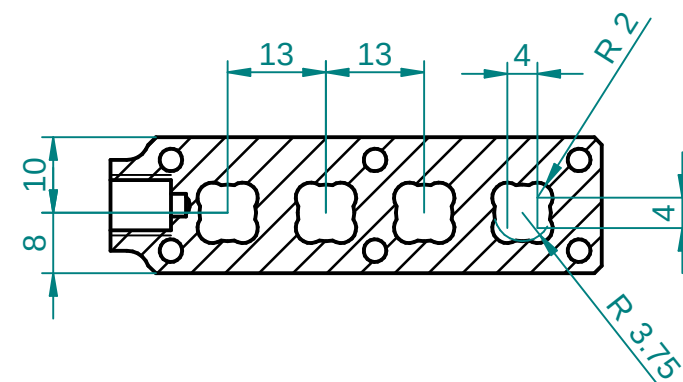
SECTION AC-AC
