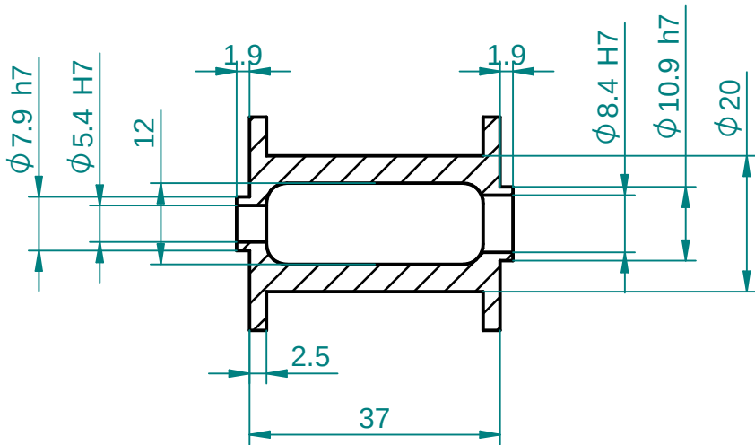
SECTION E-E
